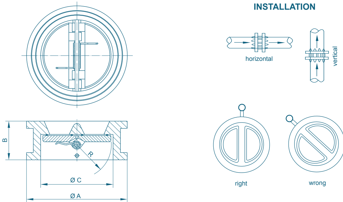
Double check valve DC
